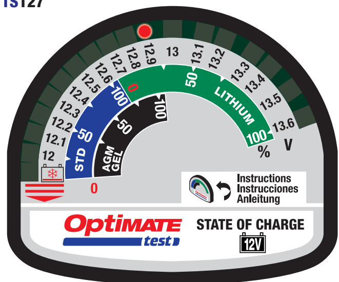
OptiMate TEST State of charge tester TS127
